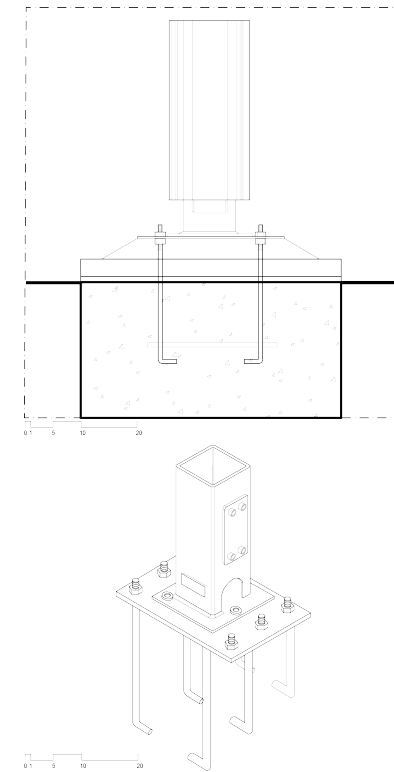
DETAIL D PERGOLA CONNECTION
